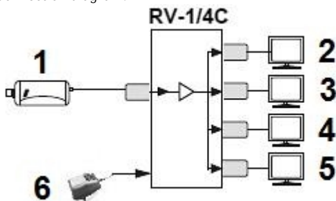
Connection diagram:
