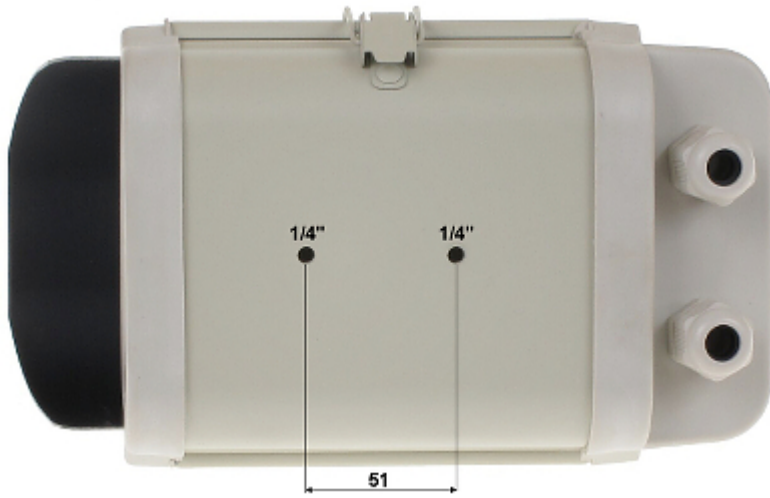
Housing with BR-300TP bracket (bracket is sold separately):
