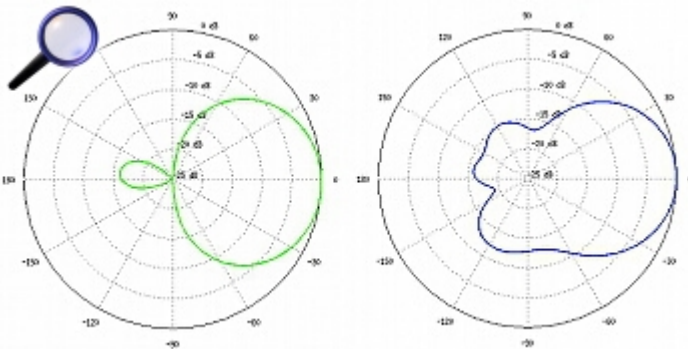
Polar pattern for vertical polarization (respectively horizontal and vertical plane):
