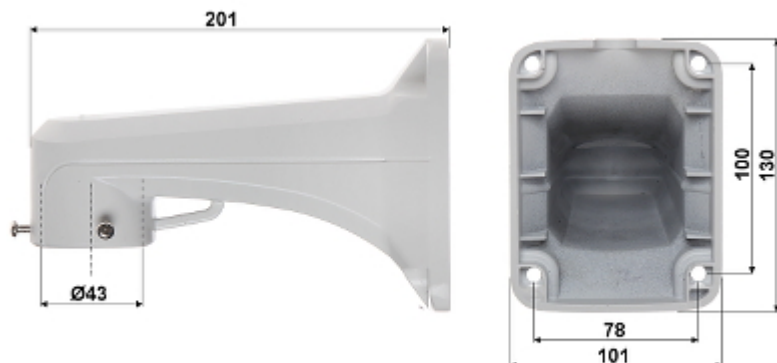
Bracket dimensions:
