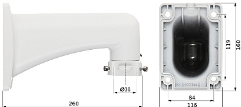
Camera dimensions:
