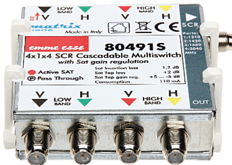
Connectors view:
