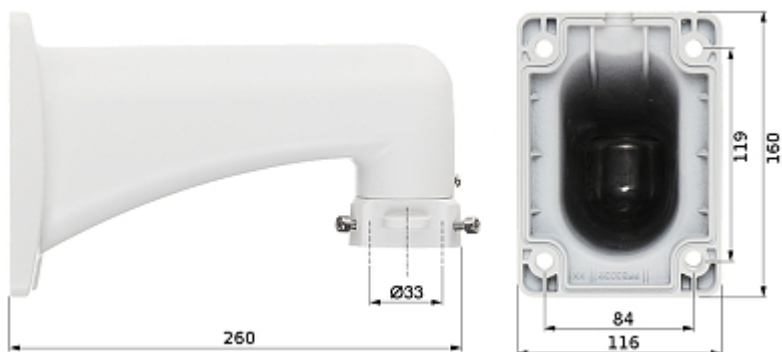
Camera dimensions:
