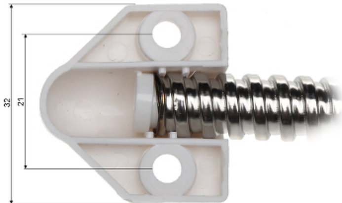
Mounting dimensions:
