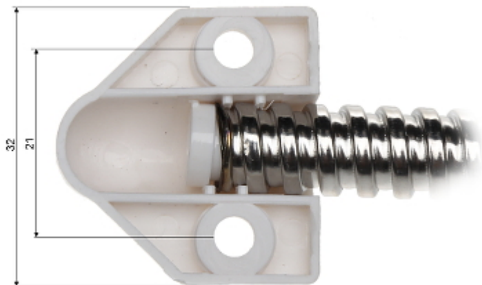
Mounting dimensions:
