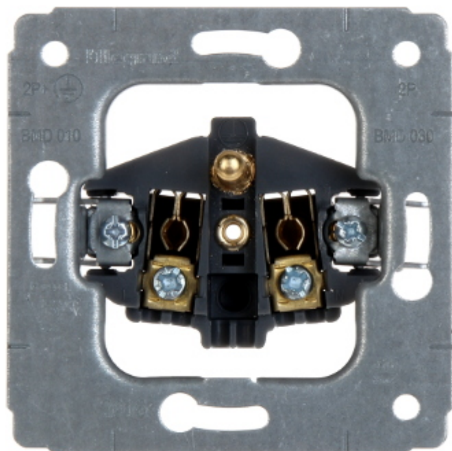
Rear view:
