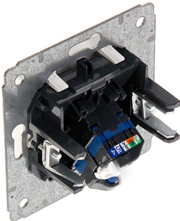
Rear view:
