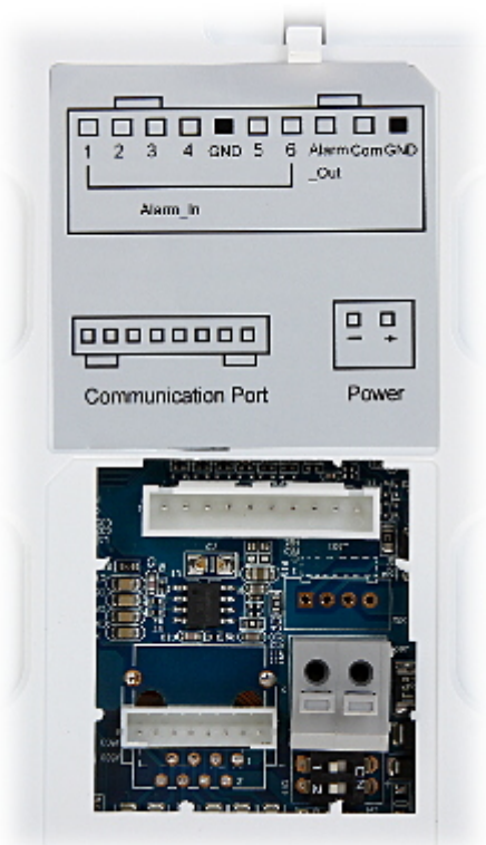
Flush-mounting box included in the set:
