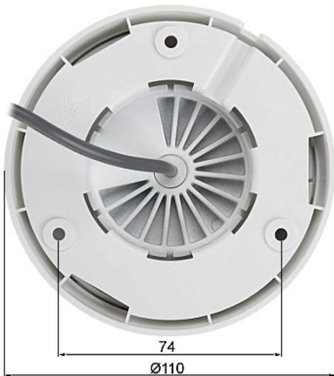
Camera dimensions:
