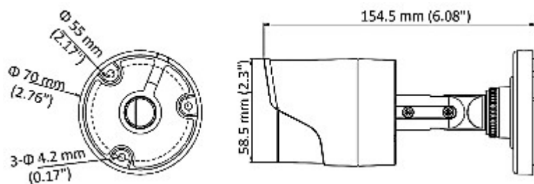
Camera dimensions:
