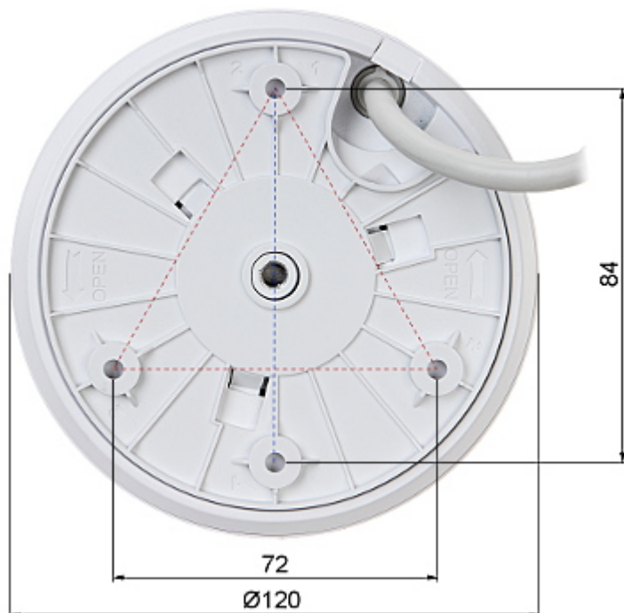
Camera dimensions:
