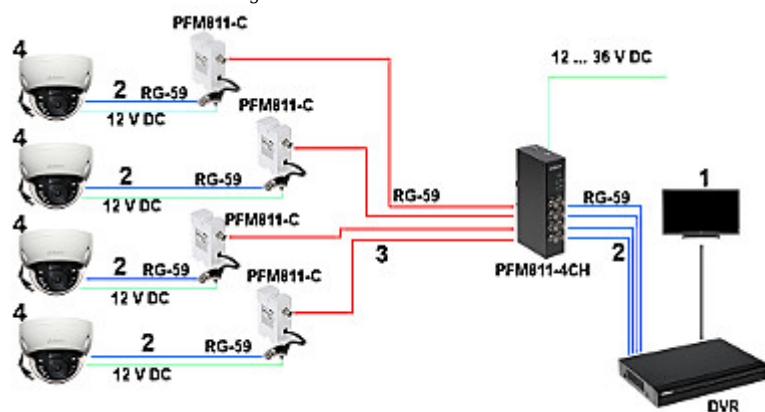
Transmission schematic diagram:
