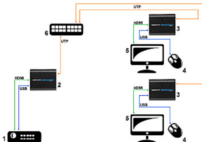
Connection schematic diagram:
