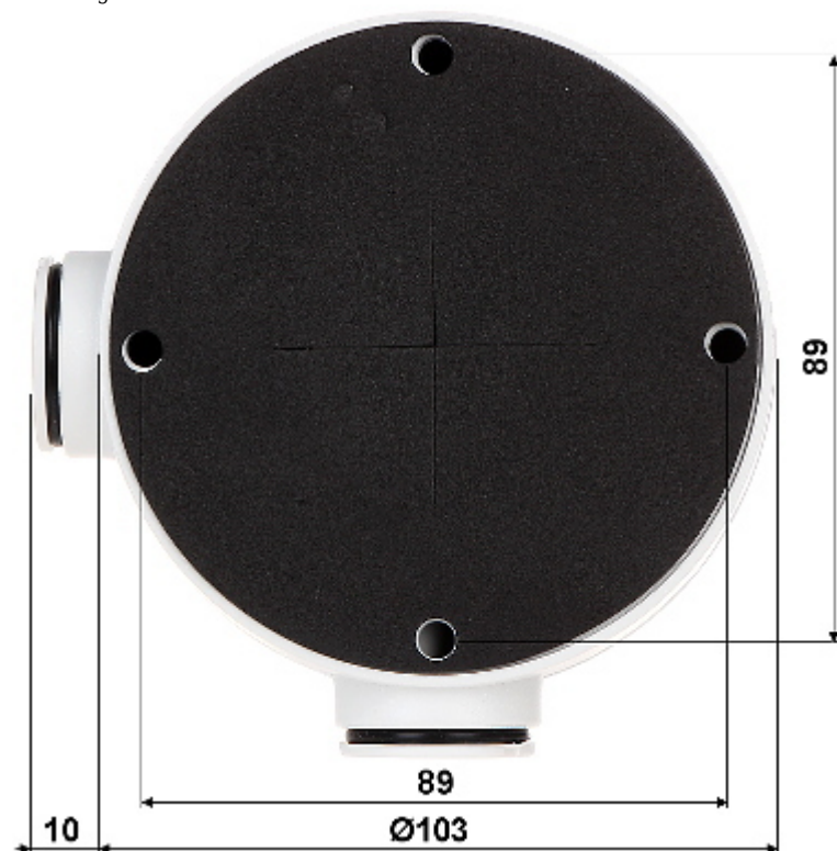
Camera dimensions:
