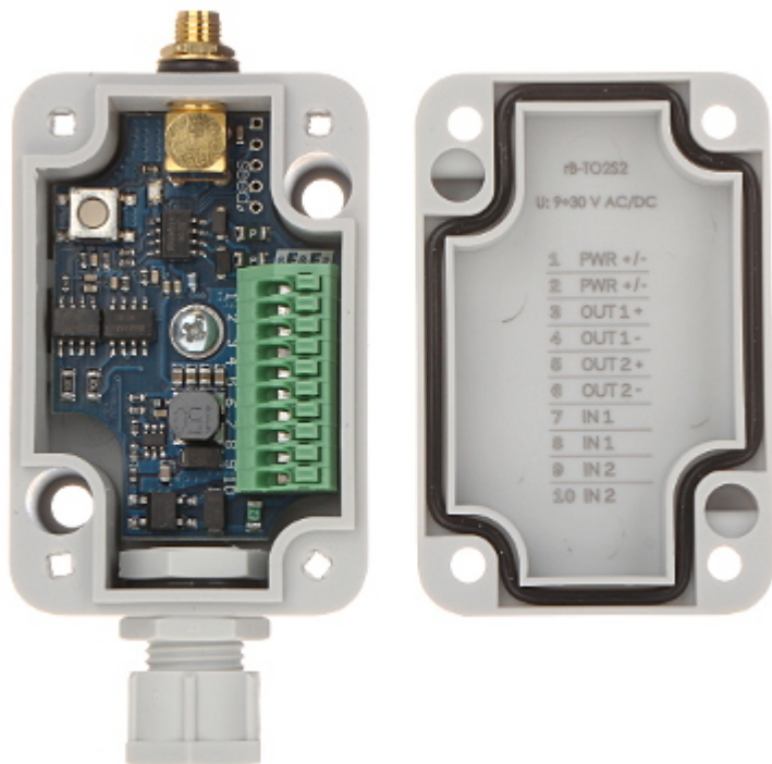
Antenna connector:
