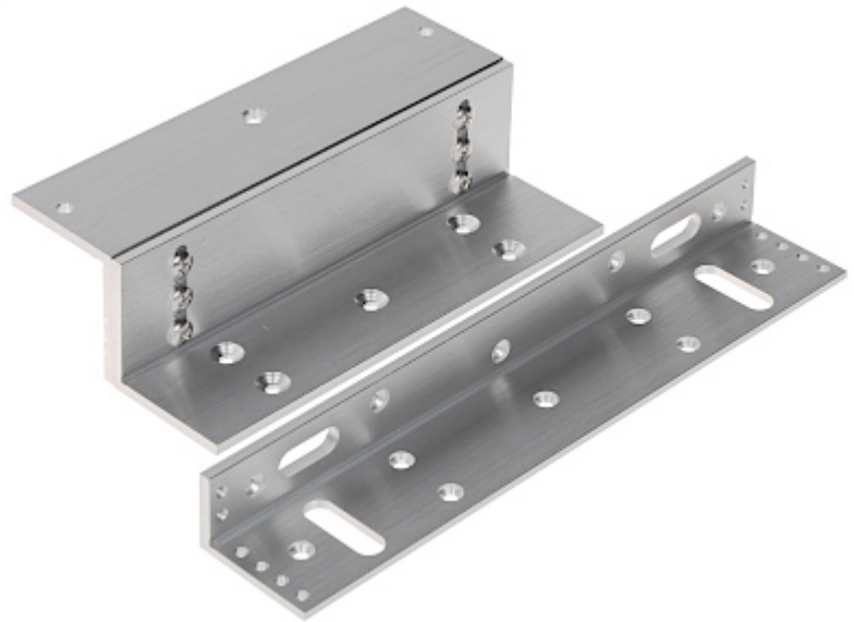
Z-bracket and L-bracket set for the ASF280A / ASF280B electromagnetic lock with load capacity of 280 kg.
