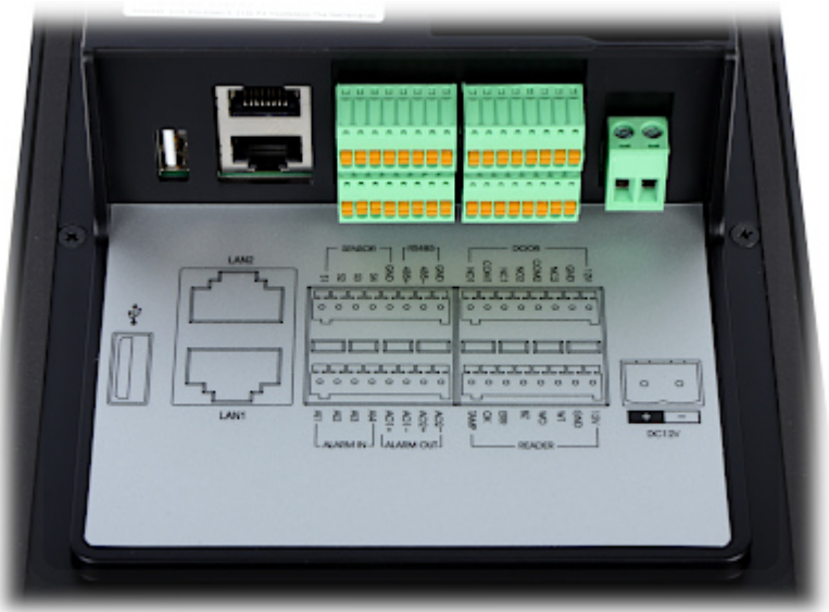
Connectors view:
