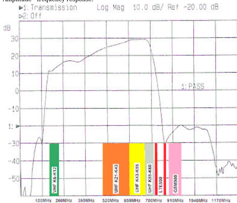
Amplitude - frequency response:
