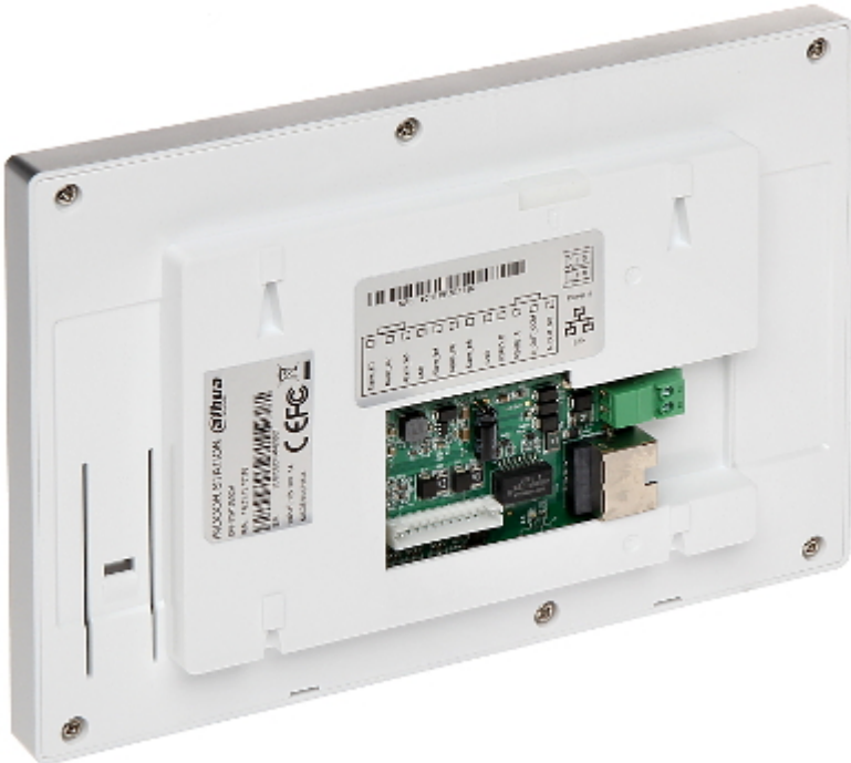
Connectors view:
