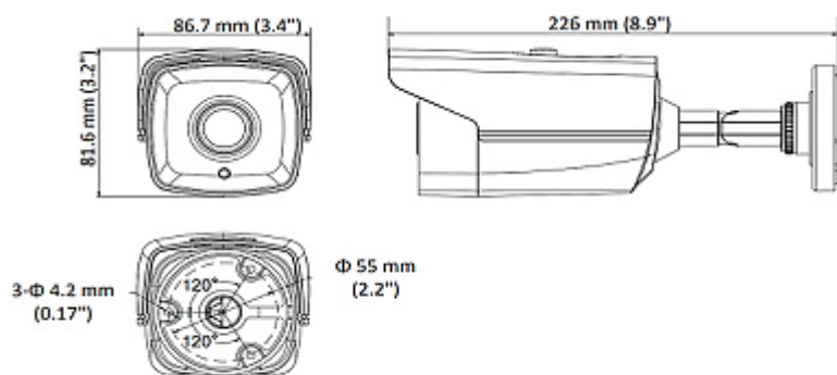
Camera dimensions:
