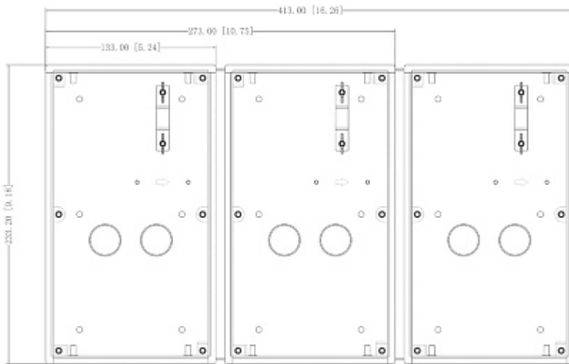
Dimensions with 3 elements combined - back side:
