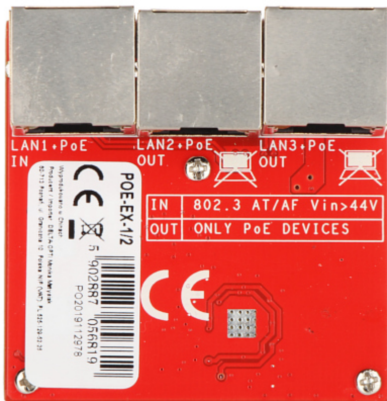
Bottom view:
