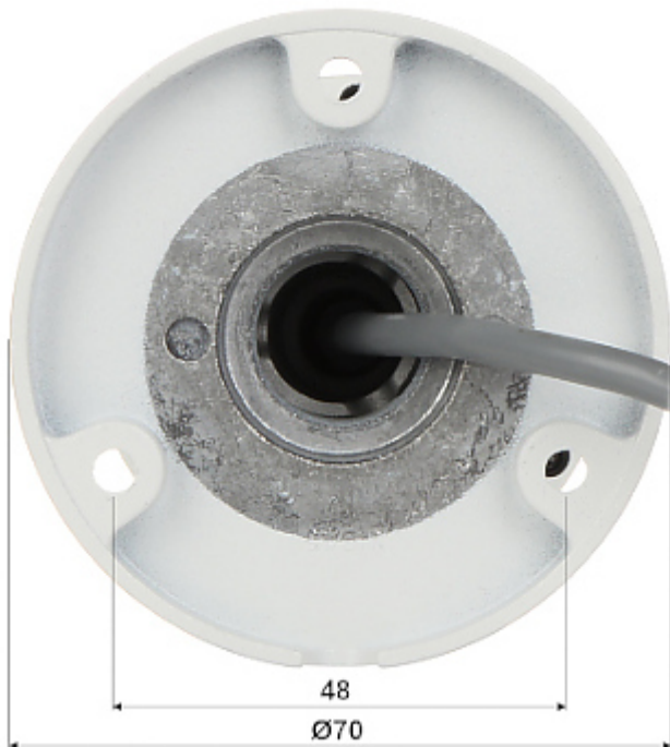
Camera dimensions:
