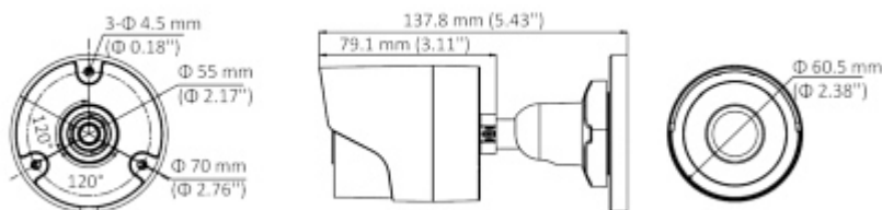
Camera dimensions:
