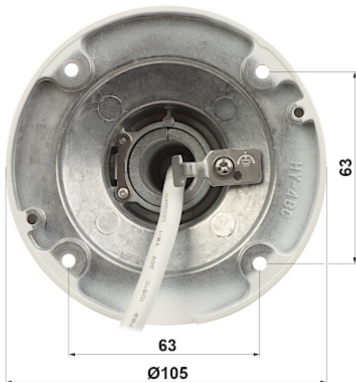
Camera dimensions:
