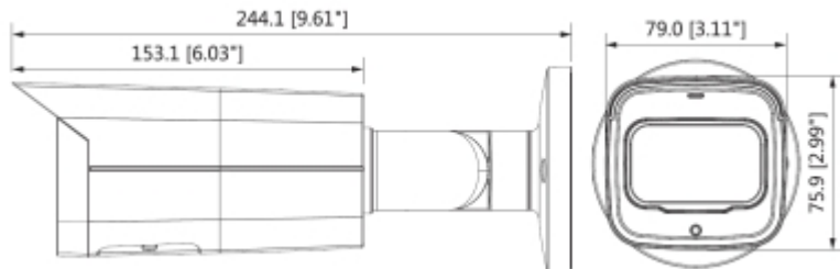
Camera dimensions:
