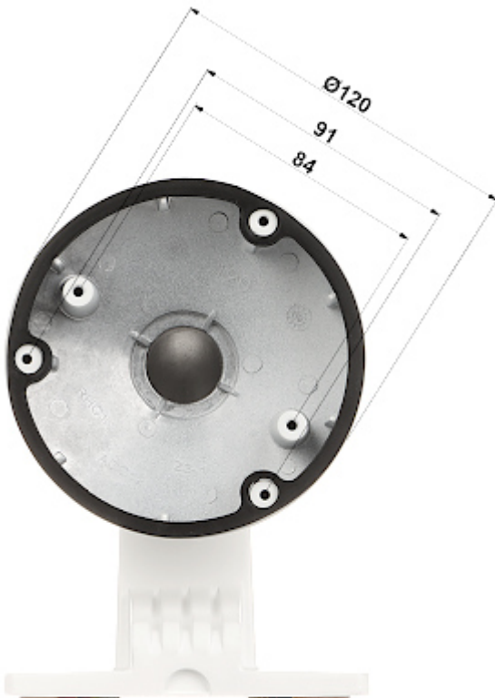
Bracket dimensions:
