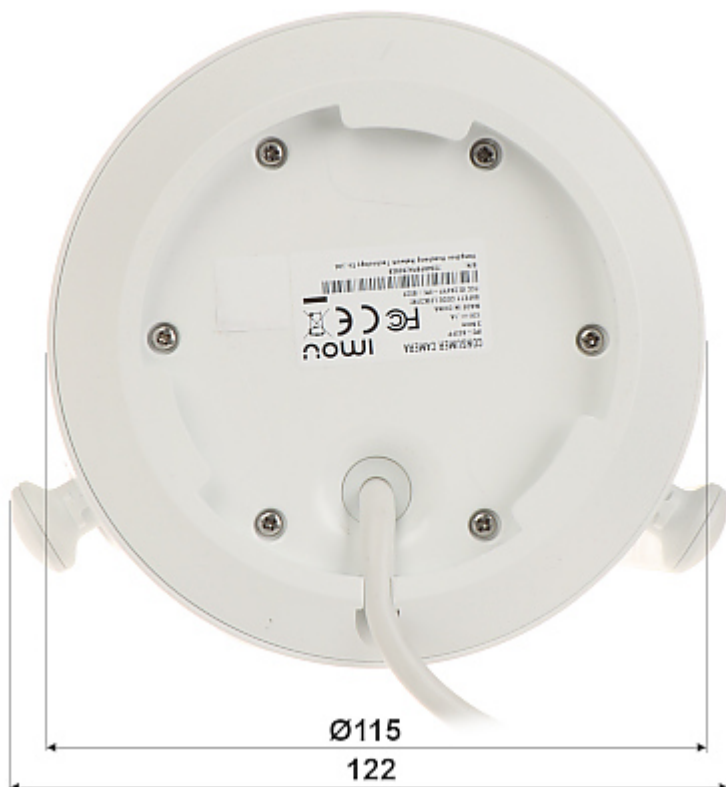
Mounting dimensions:
