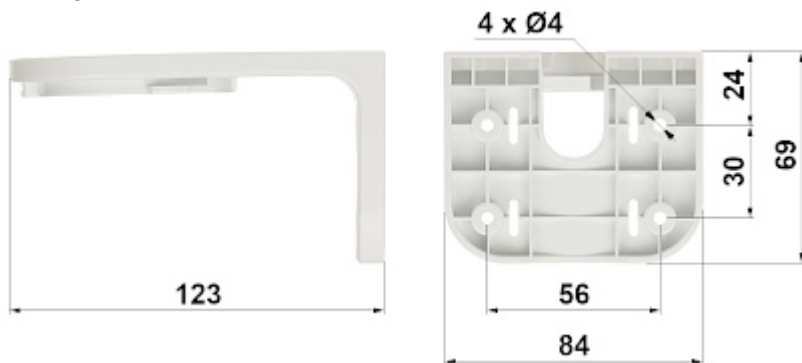
Camera connectors:
