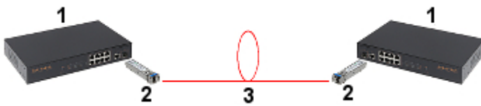
Connection diagram:
