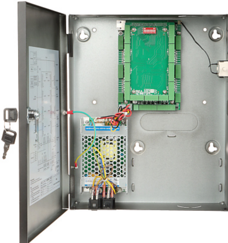
Internal view of the housing
