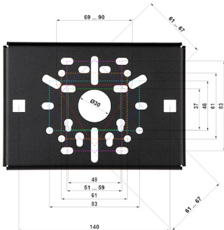
Mounting dimensions:
