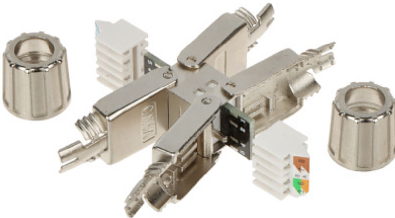
Internal view:
