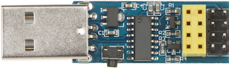
USB connector:
