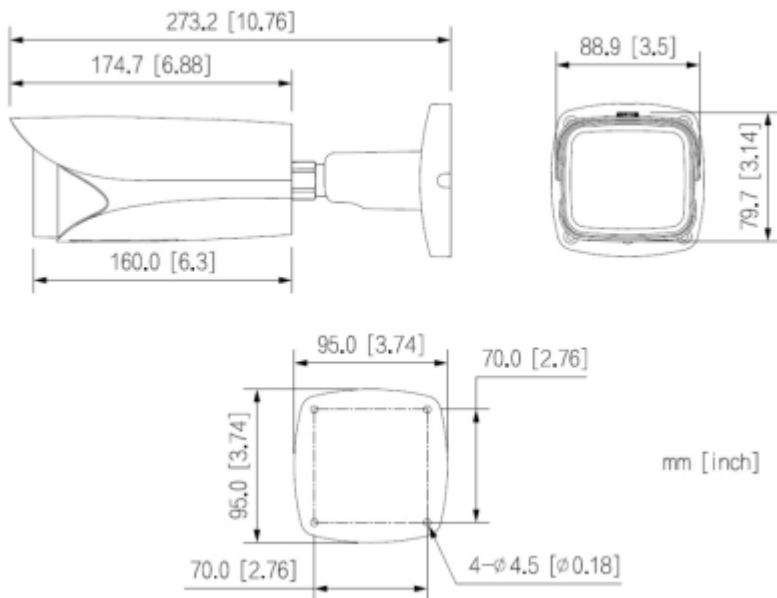
Camera dimensions:
