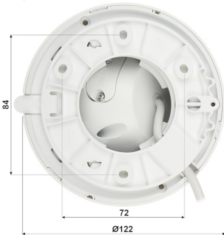
Mounting dimensions
