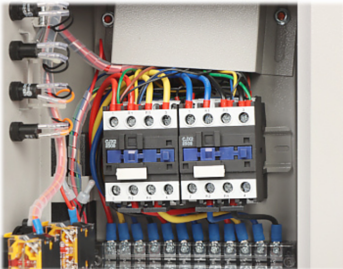
Internal view of the housing:
