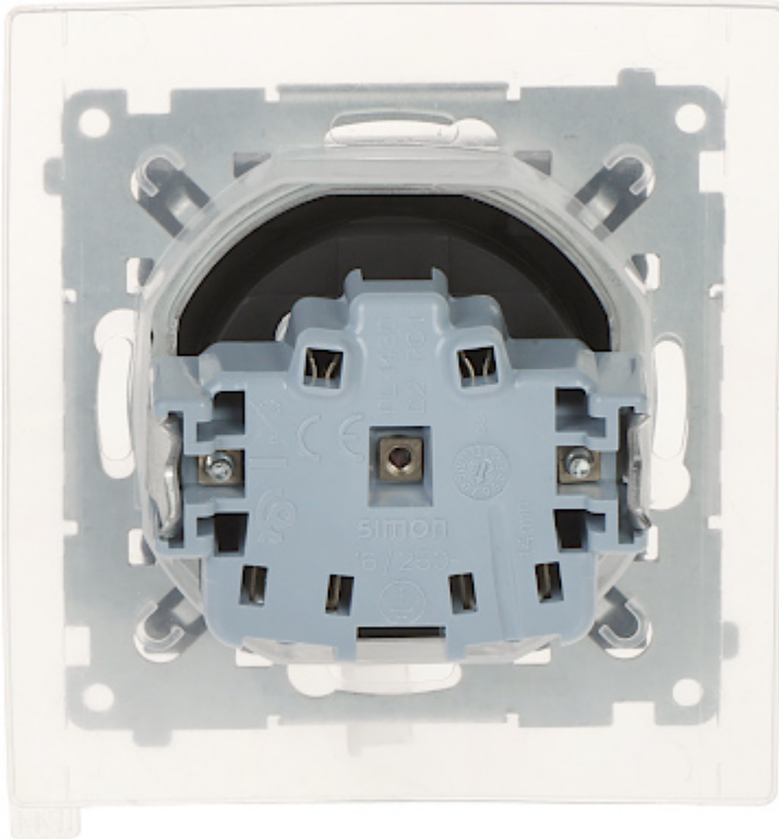
Connectors view:
