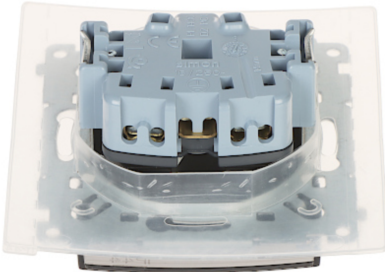
Connectors view:
