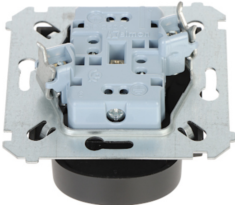
Connectors view:
