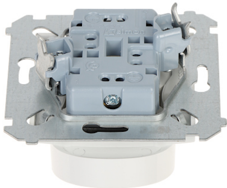
Connectors view:
