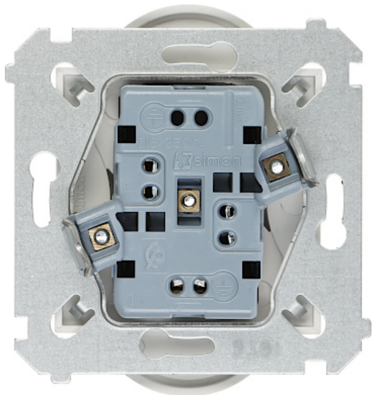
Connectors view:
