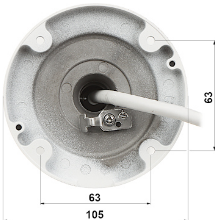
Camera dimensions:
