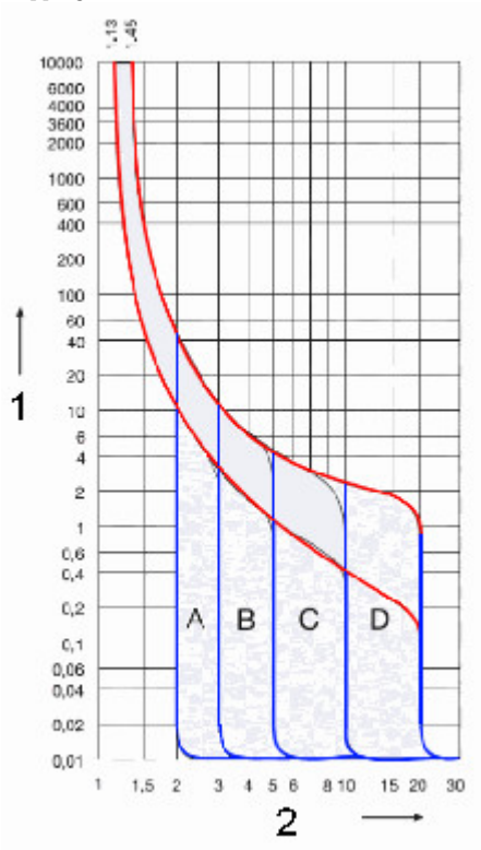
Tripping curves
