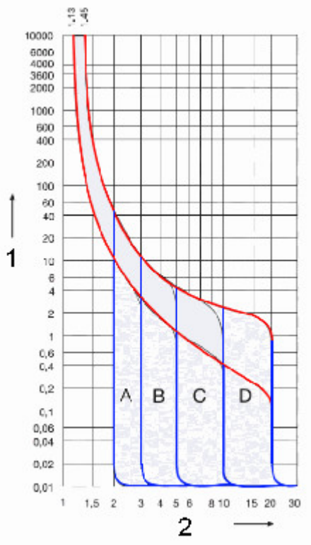
Tripping curves:
