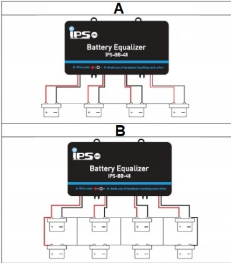
A - 4 batteries in a 48V (4*12V) system B - Multiple sets of batteries
