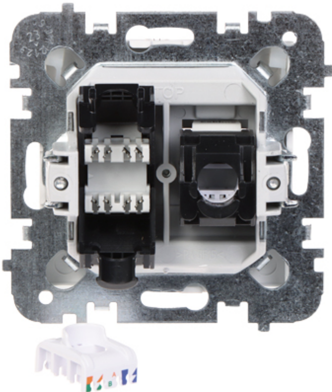
Connectors view:
