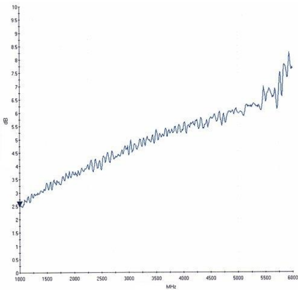
The TRI-LAN-240 cable matching in frequency response:
