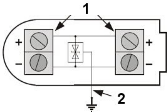
Connection diagram:
