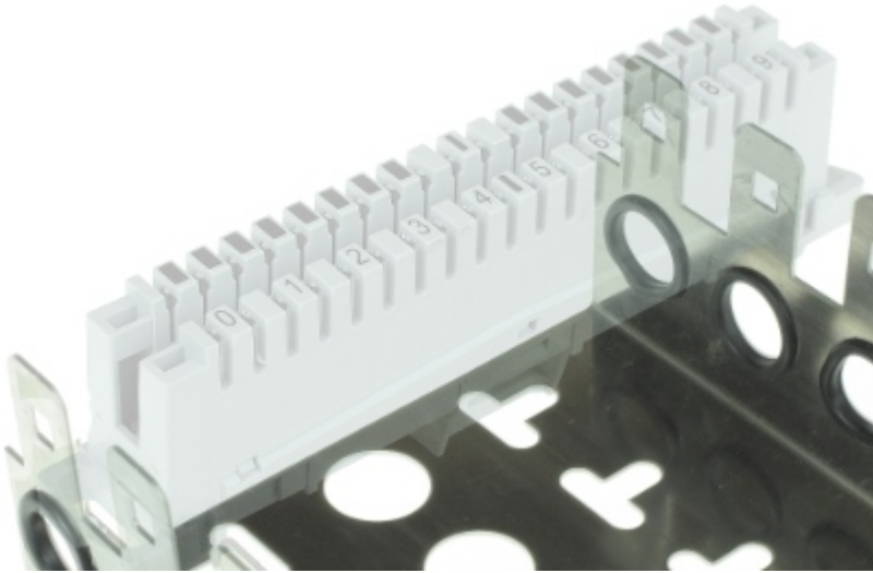
Twisted-pair cable mounting using a KRONE impact tool (ZAC/LSA-P):
