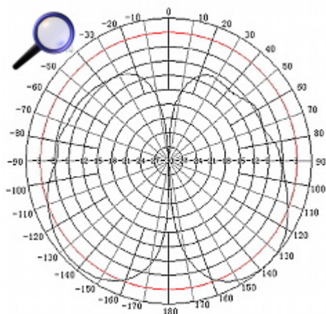
Antenna characteristics:
